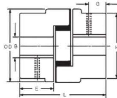
SX (2 hubs plus spider element)
