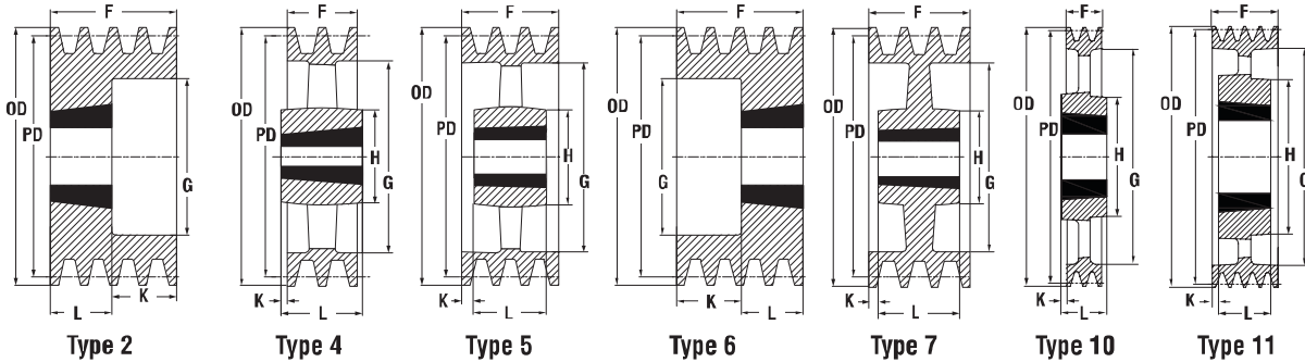
Pulley Groove Dimensions (ISO Standard)
