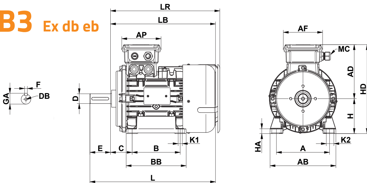
IMB3 - Ex db eb - Dimensions in mm
